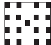
Springstep IV Foam Block Layout 3" x 3" x 3/4" (17 required)
